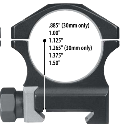
Ultralite™ aluminum/titanium rings (30mm & 34mm)
