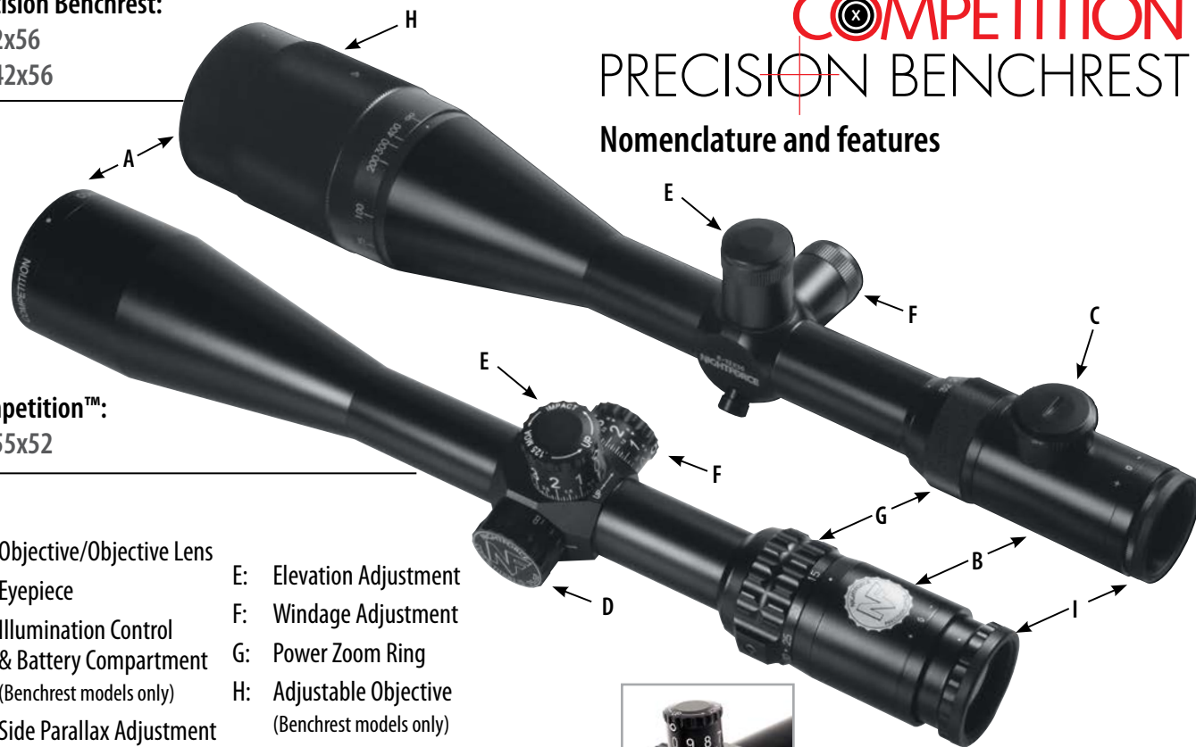
Competition™ high-visibility windage and elevation adjustments
